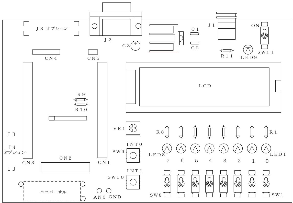
OAKS-LCD Board
